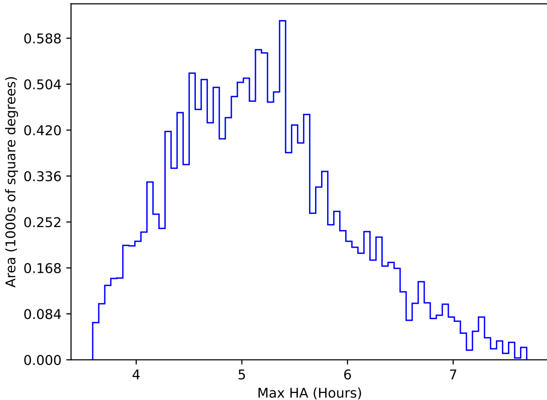
reweight_plane_v3.3_10yrs WFD all bands: Max HA
