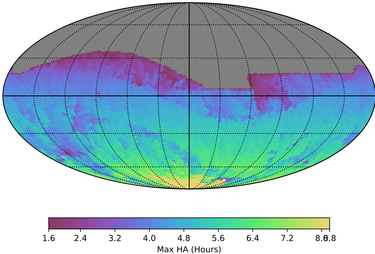
reweight_plane_v3.3_10yrs All sky z band: Max HA
