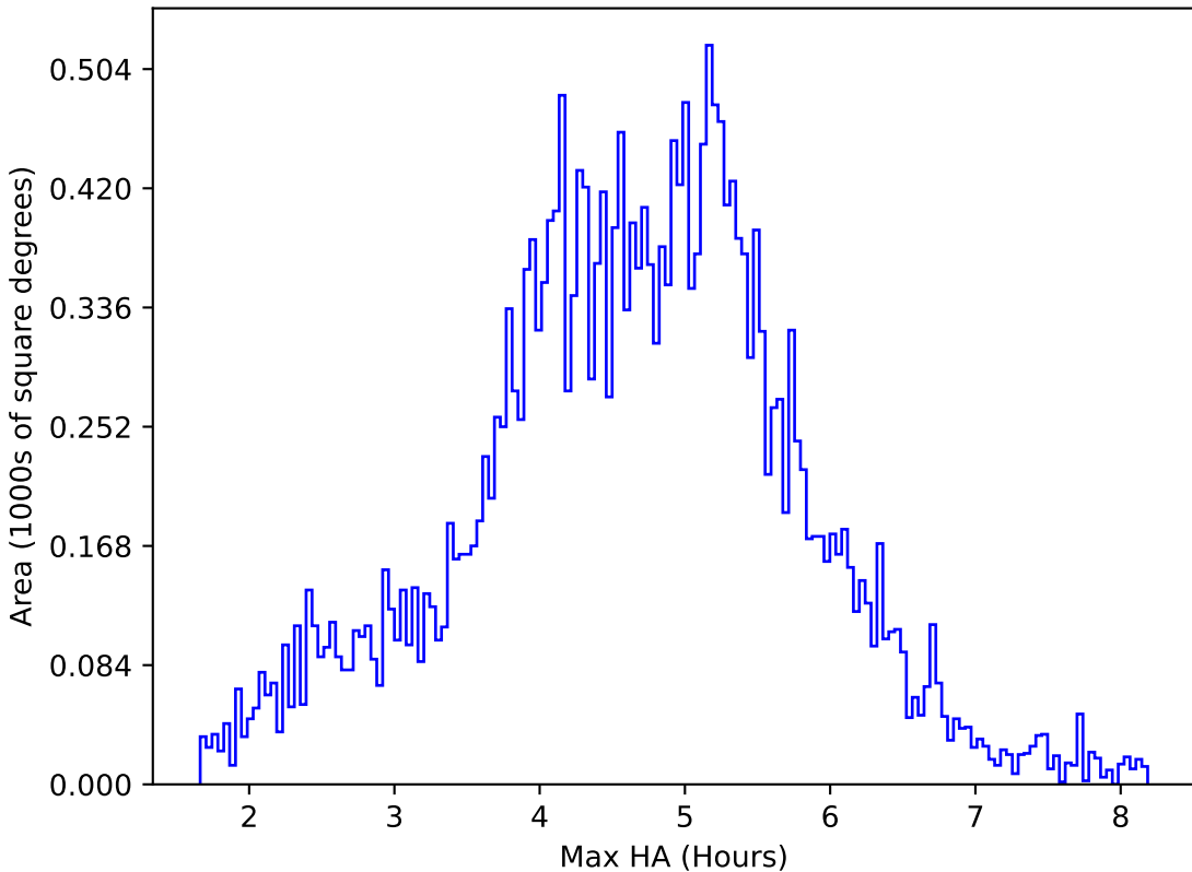
reweight_plane_v3.3_10yrs All sky z band: Max HA
