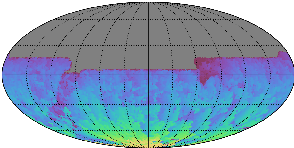
reweight_plane_v3.3_10yrs All sky y band: Max HA
