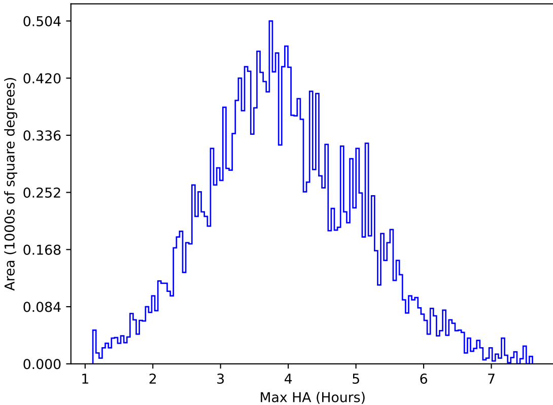
reweight_plane_v3.3_10yrs All sky u band: Max HA
