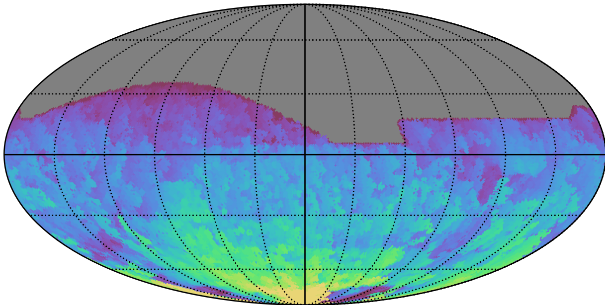
reweight_plane_v3.3_10yrs All sky r band: Max HA
