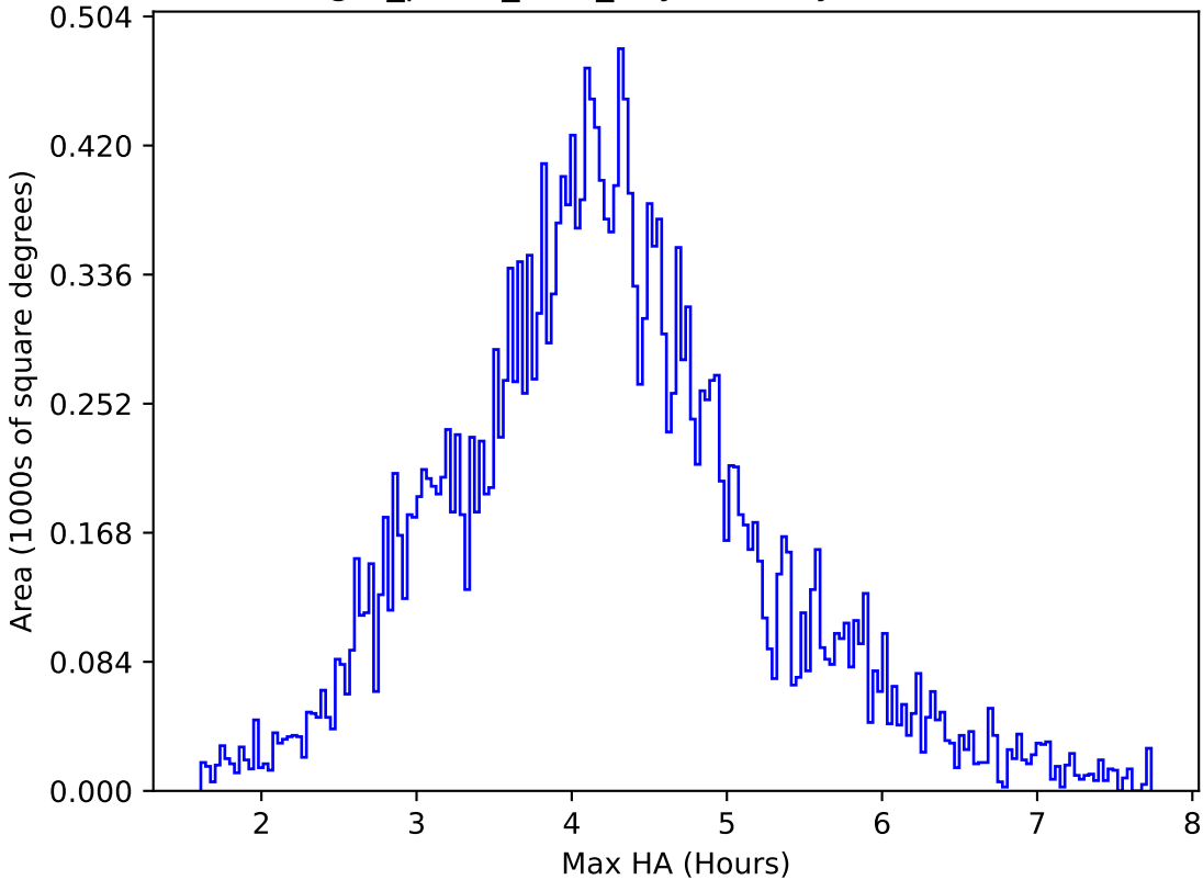
reweight_plane_v3.3_10yrs All sky r band: Max HA
