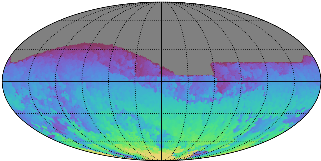
reweight_plane_v3.3_10yrs All sky i band: Max HA
