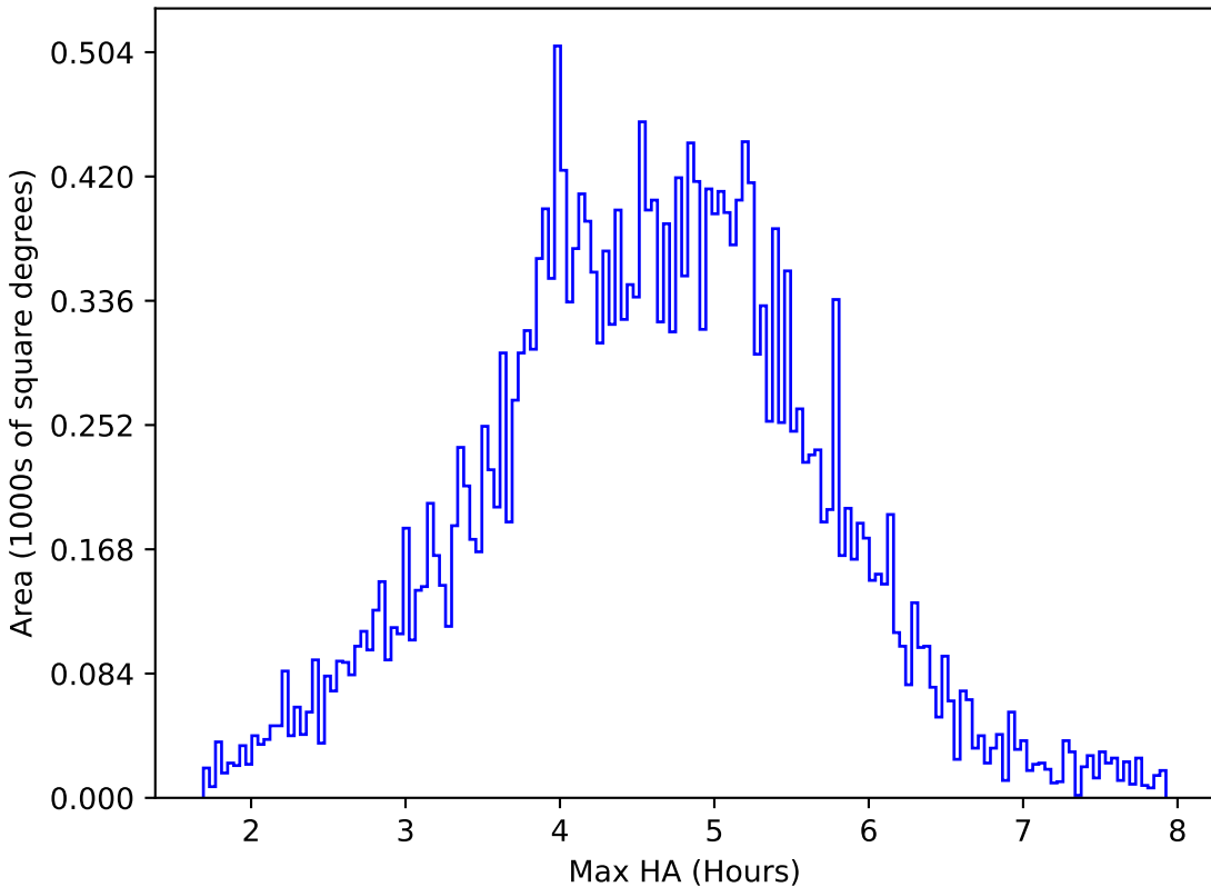
reweight_plane_v3.3_10yrs All sky i band: Max HA
