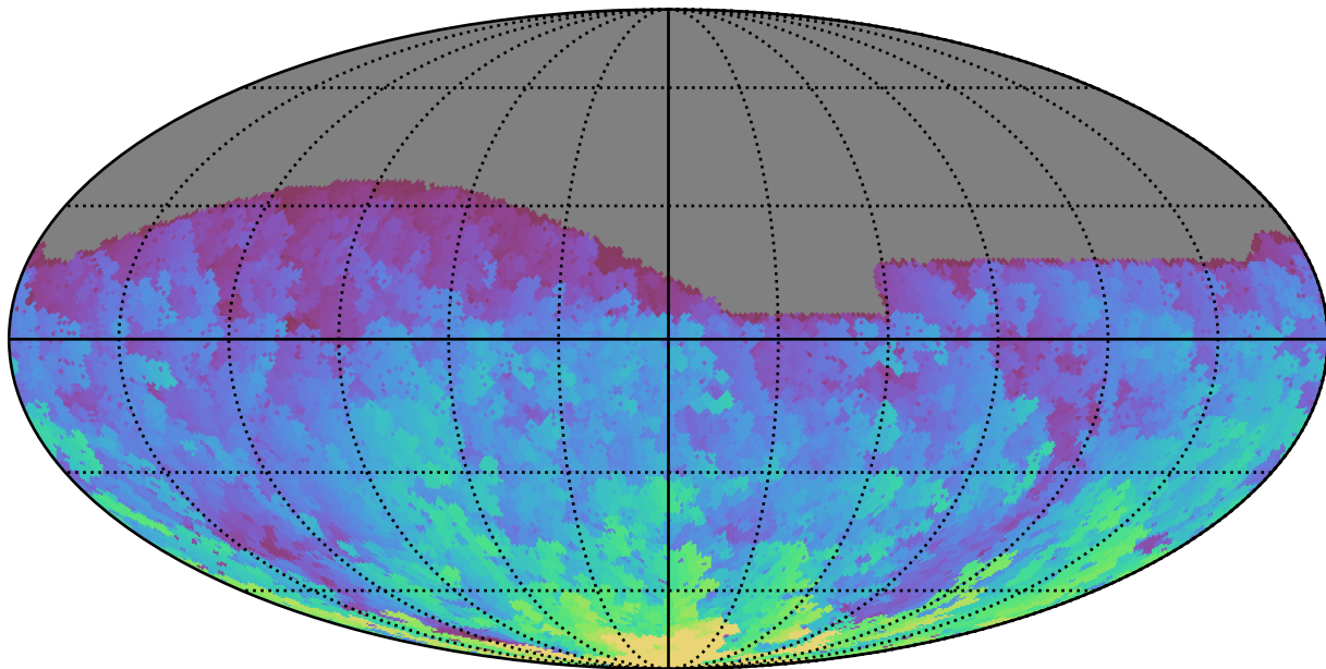
reweight_plane_v3.3_10yrs All sky g band: Max HA
