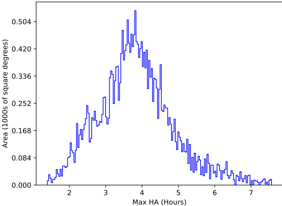
reweight_plane_v3.3_10yrs All sky g band: Max HA
