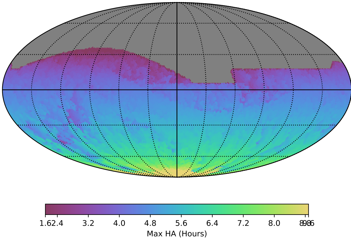
reweight_plane_v3.3_10yrs All sky all bands: Max HA
