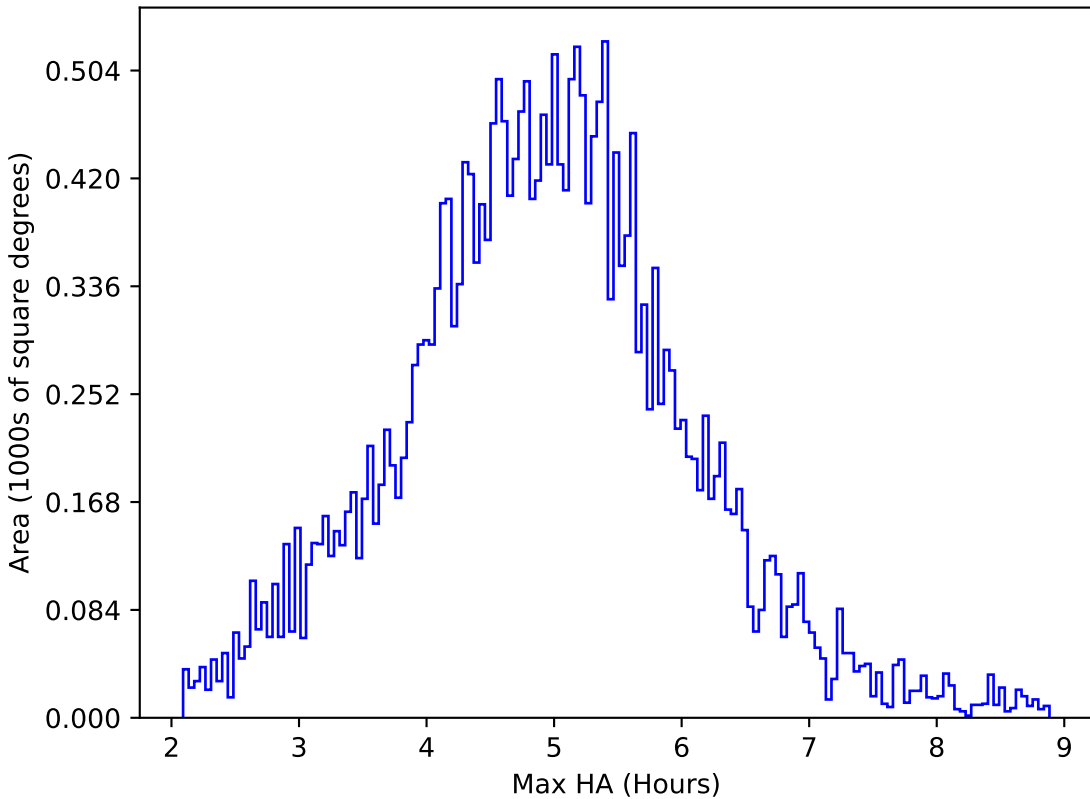
reweight_plane_v3.3_10yrs All sky all bands: Max HA
