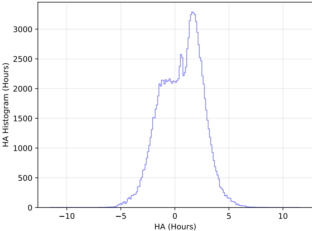
reweight_plane_v3.3_10yrs WFD u band: HA Histogram
