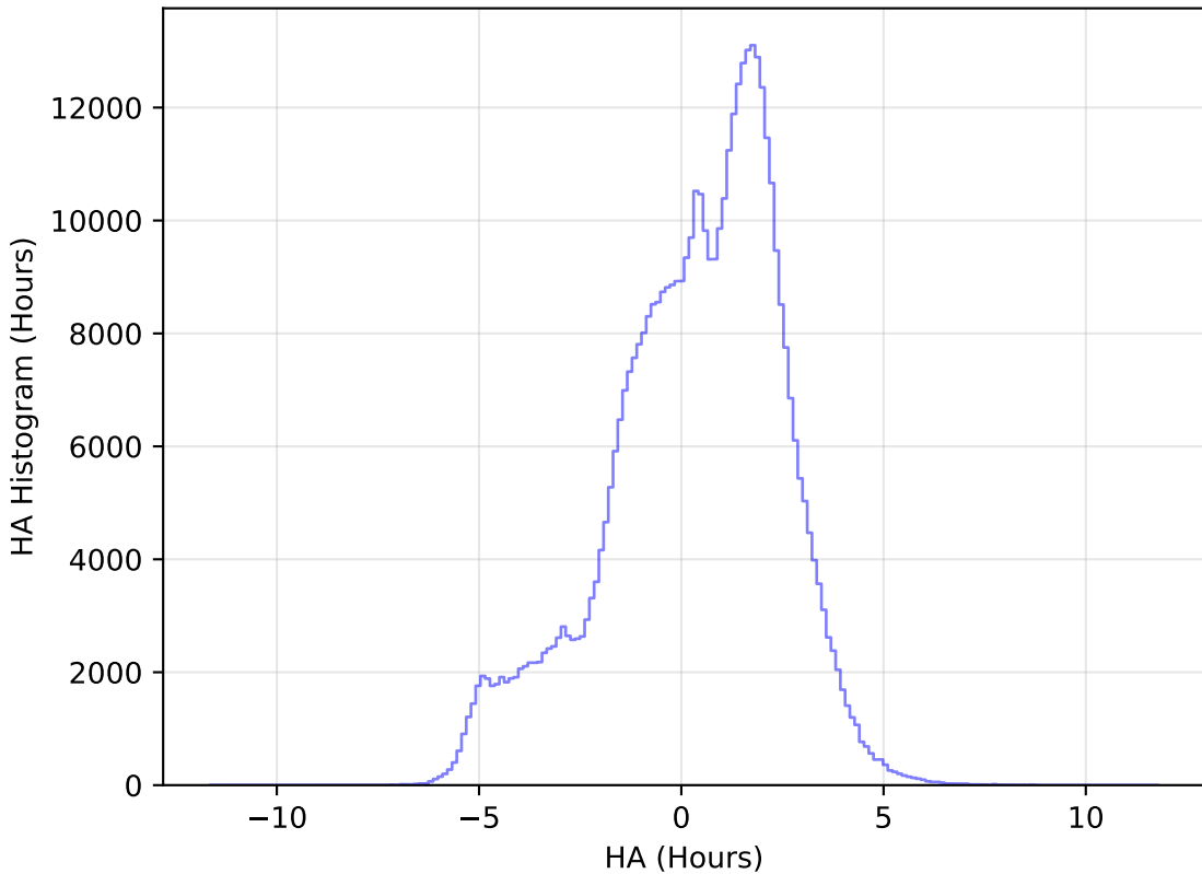
reweight_plane_v3.3_10yrs WFD r band: HA Histogram
