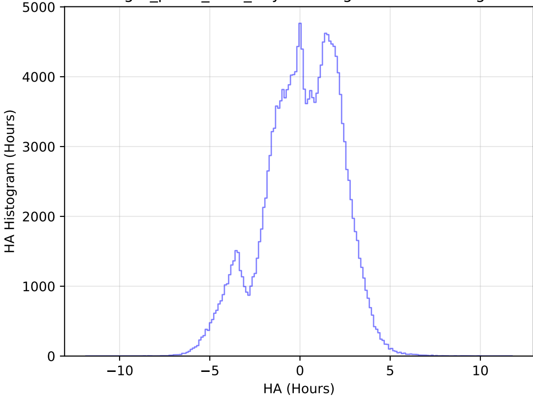
reweight_plane_v3.3_10yrs WFD g band: HA Histogram
