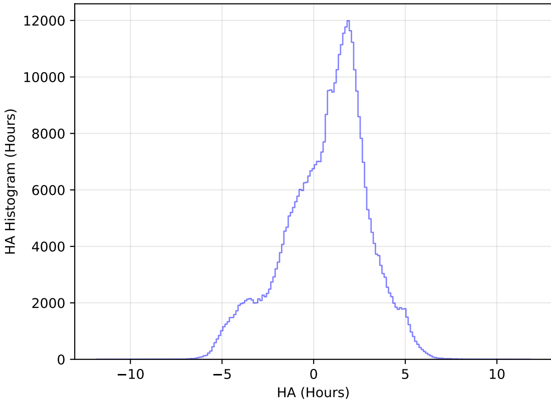
reweight_plane_v3.3_10yrs All sky z band: HA Histogram
