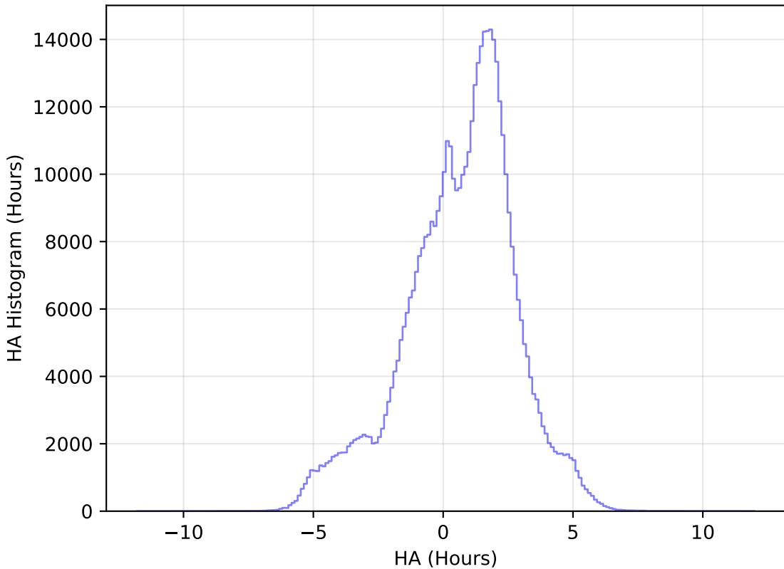
reweight_plane_v3.3_10yrs All sky i band: HA Histogram
