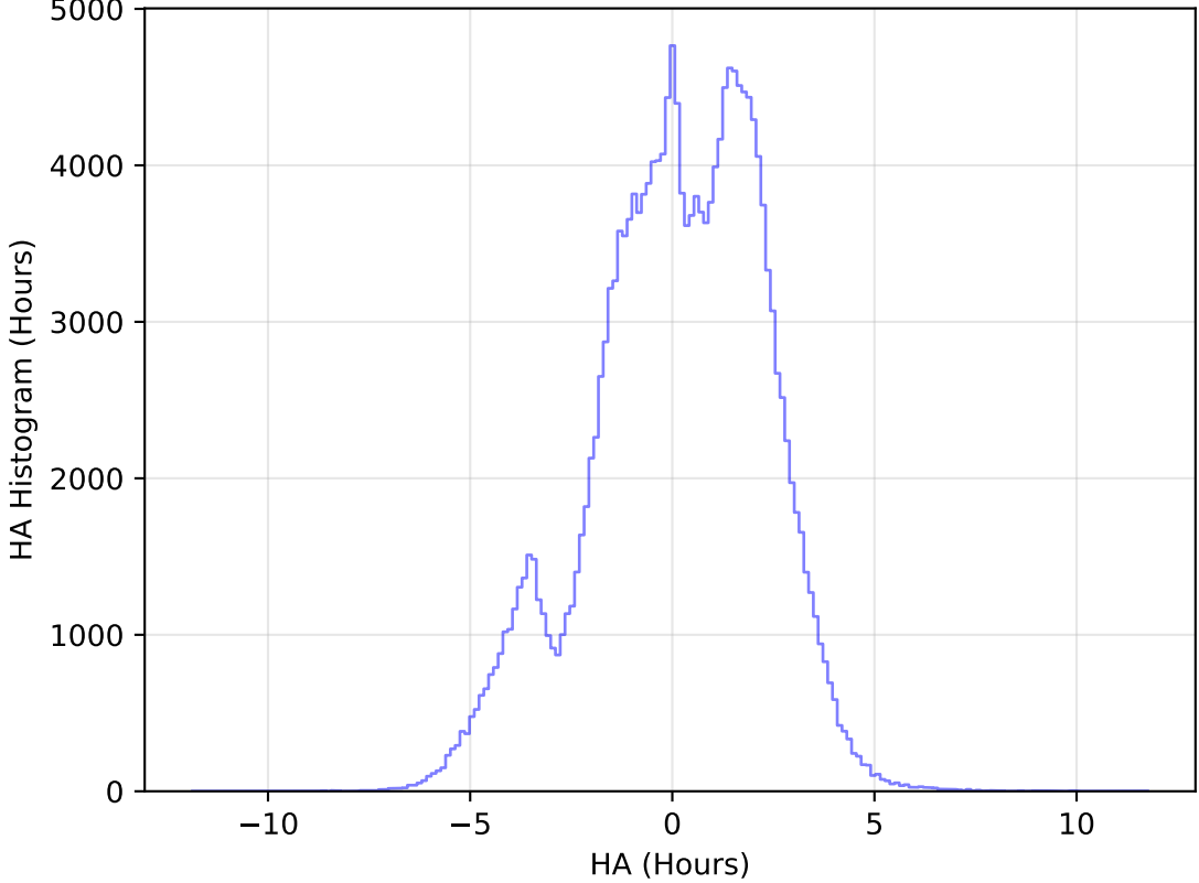
reweight_plane_v3.3_10yrs All sky g band: HA Histogram
