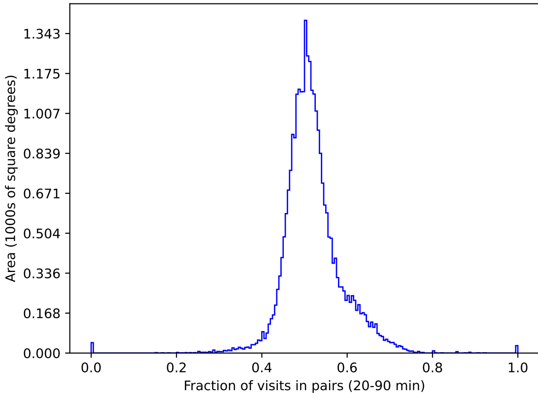
reweight_plane_v3.3_10yrs gri All sky: Fraction of visits in pairs (20-90 min)
