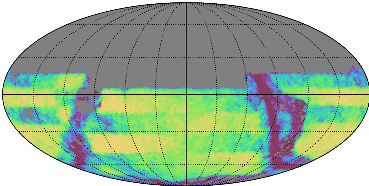
reweight_plane_v3.3_10yrs Yr 3-4 y band: Exgal_CoaddM5
