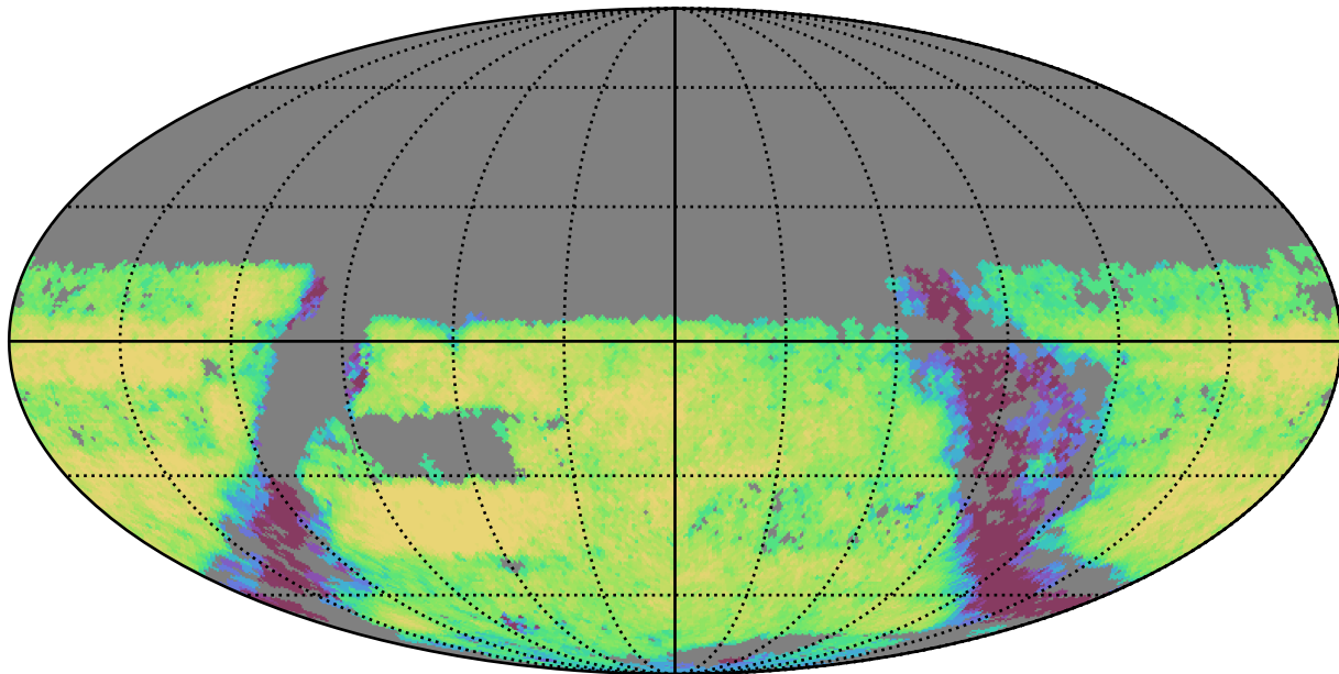
reweight_plane_v3.3_10yrs Yr 3-4 u band: Exgal_CoaddM5
