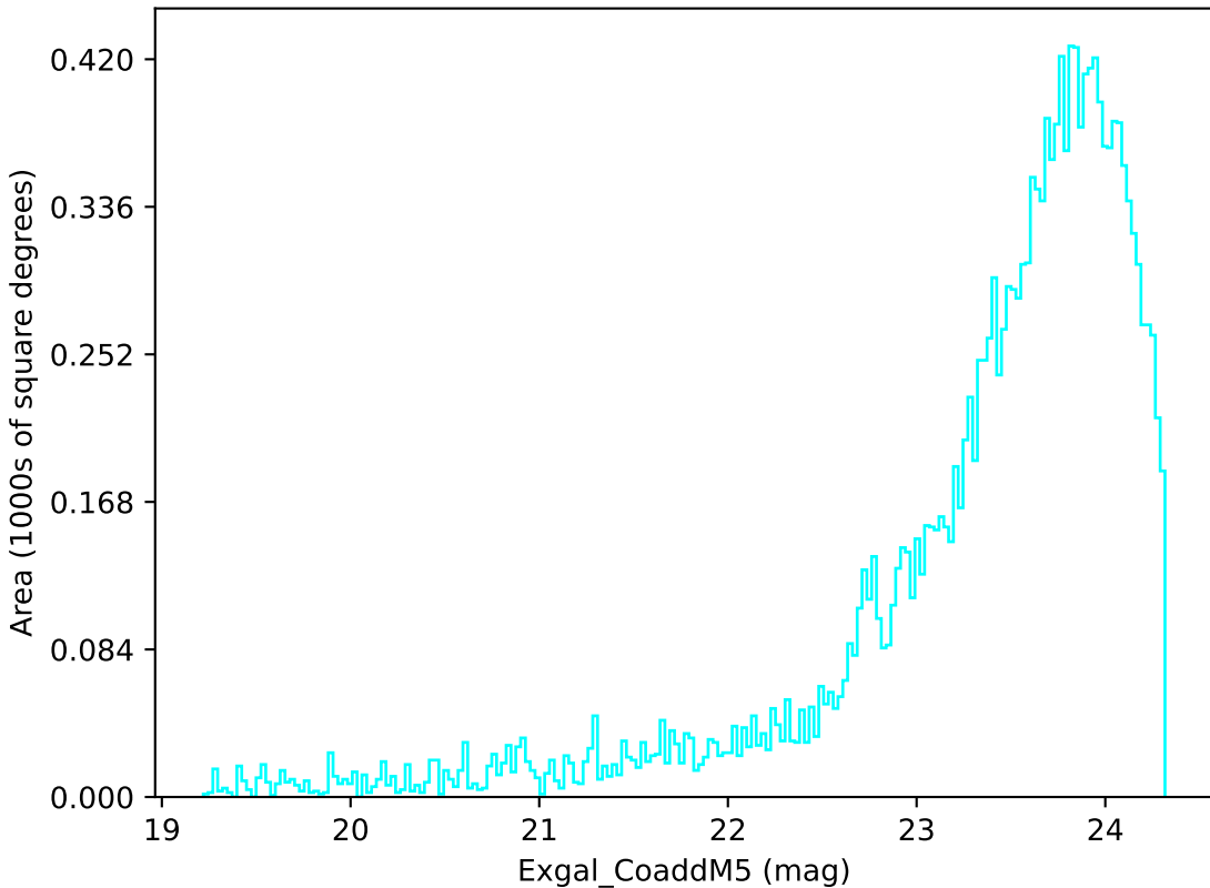
reweight_plane_v3.3_10yrs Yr 3-4 u band: Exgal_CoaddM5
