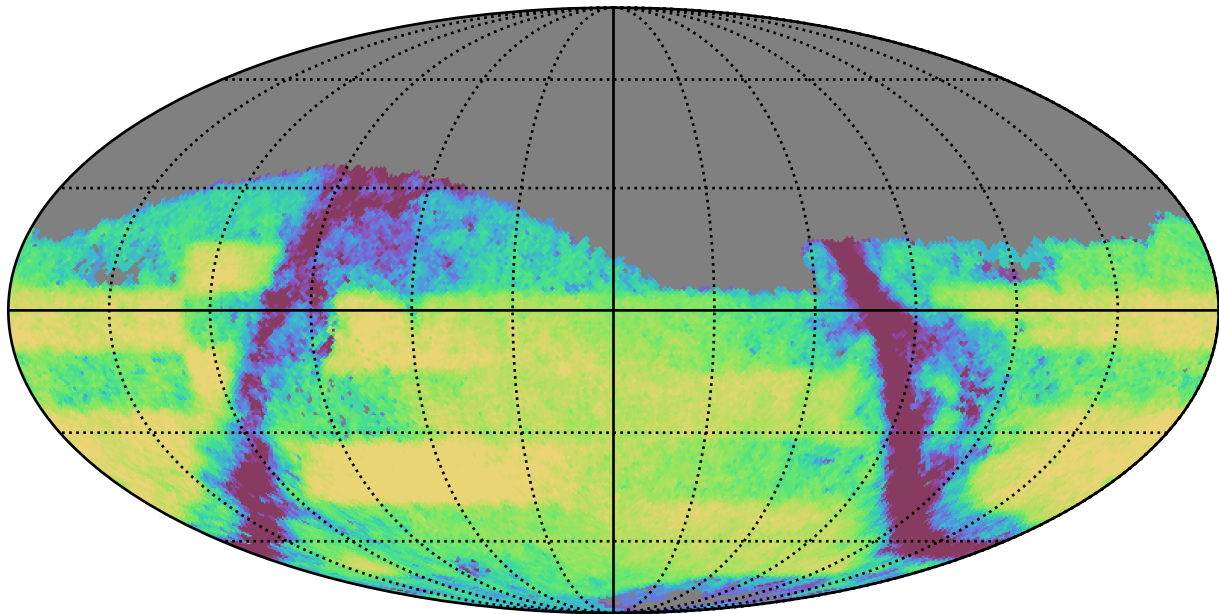
reweight_plane_v3.3_10yrs Yr 3-4 r band: Exgal_CoaddM5
