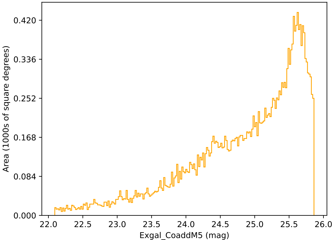
reweight_plane_v3.3_10yrs Yr 3-4 r band: Exgal_CoaddM5
