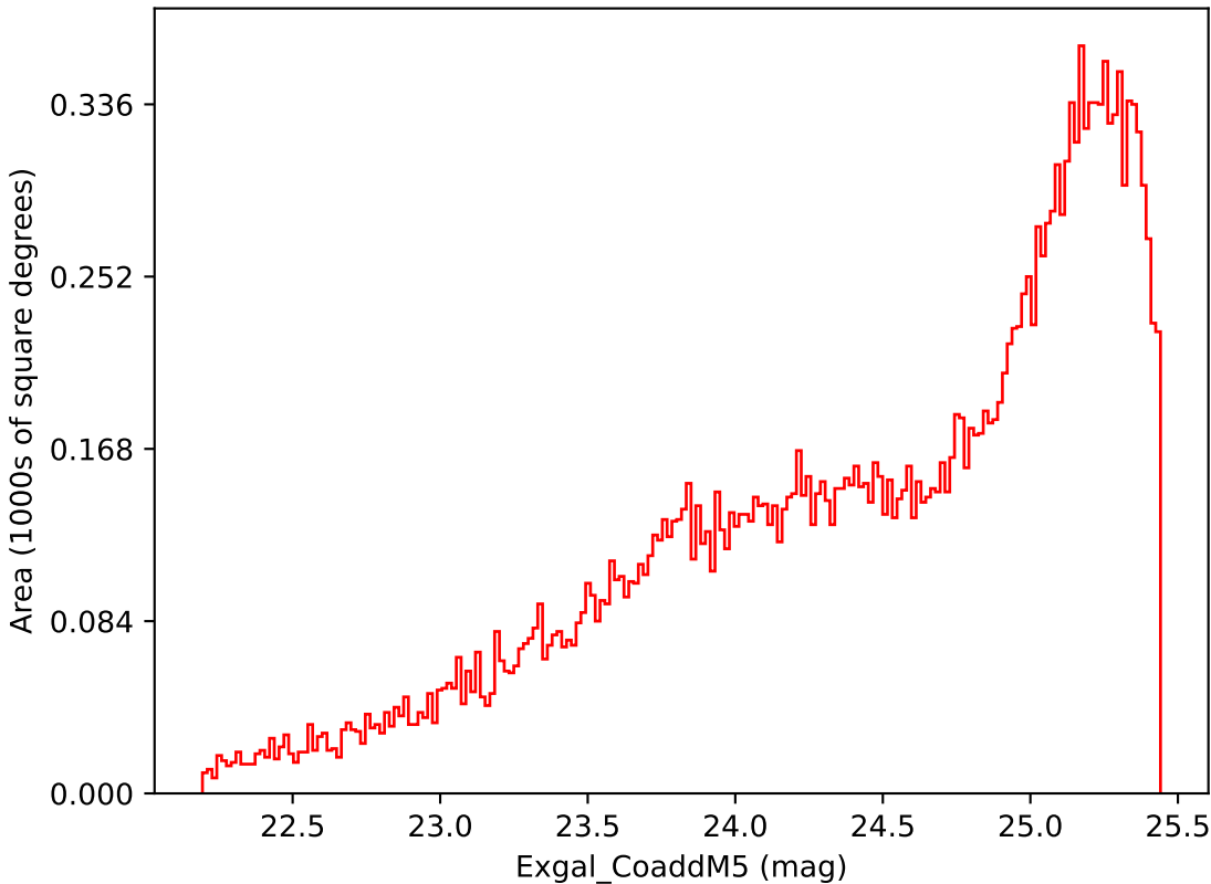
reweight_plane_v3.3_10yrs Yr 3-4 i band: Exgal_CoaddM5
