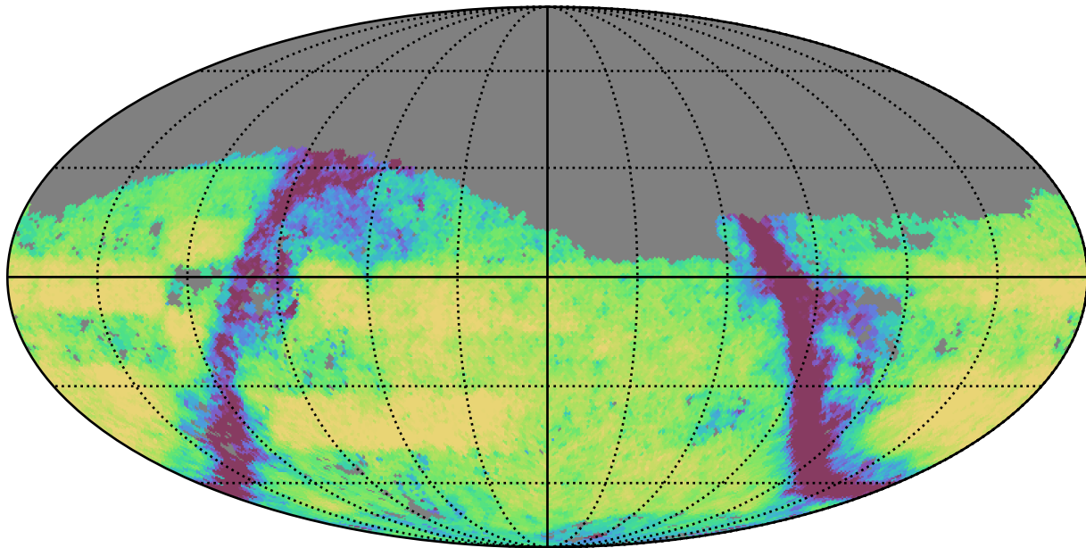
reweight_plane_v3.3_10yrs Yr 3-4 g band: Exgal_CoaddM5
