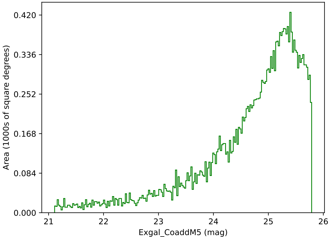
reweight_plane_v3.3_10yrs Yr 3-4 g band: Exgal_CoaddM5
