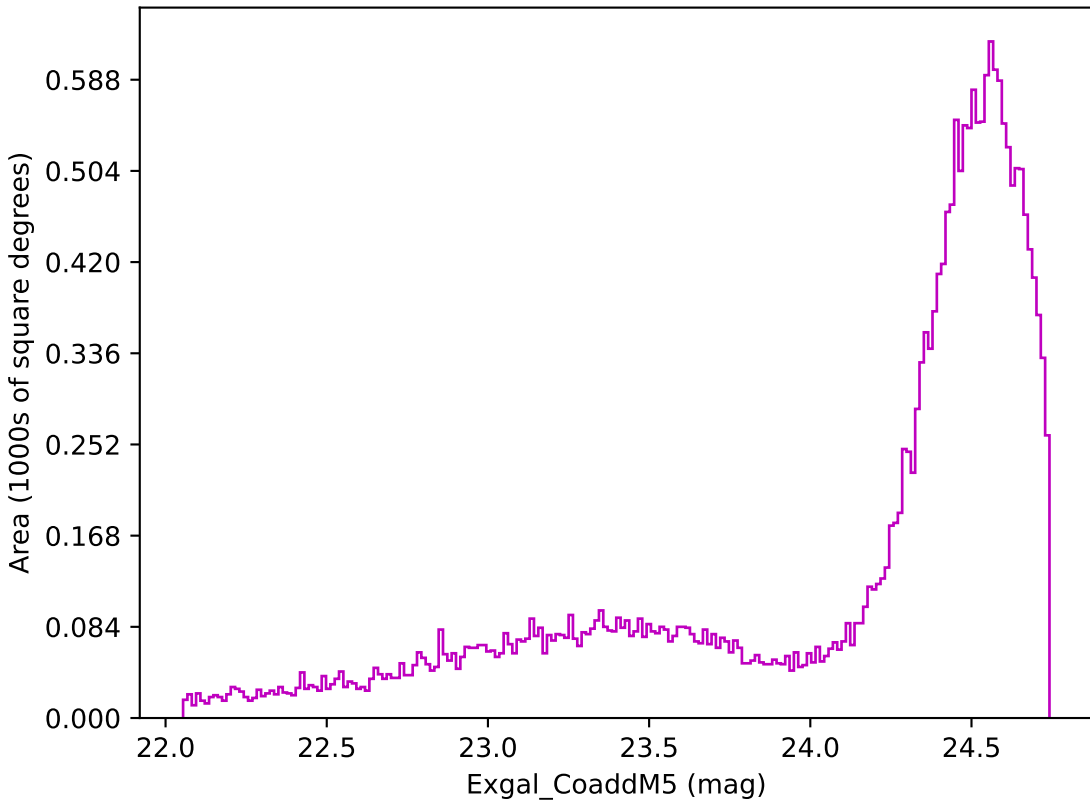
reweight_plane_v3.3_10yrs Yr 1 z band: Exgal_CoaddM5
