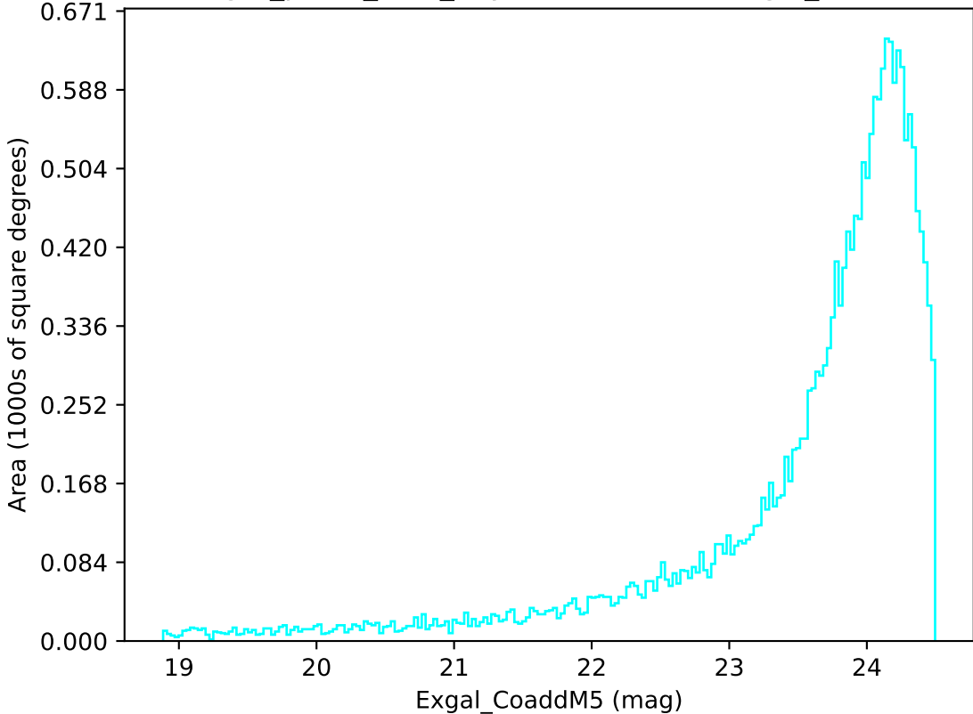
reweight_plane_v3.3_10yrs Yr 1 u band: Exgal_CoaddM5
