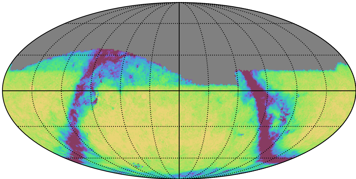
reweight_plane_v3.3_10yrs Yr 1 r band: Exgal_CoaddM5
