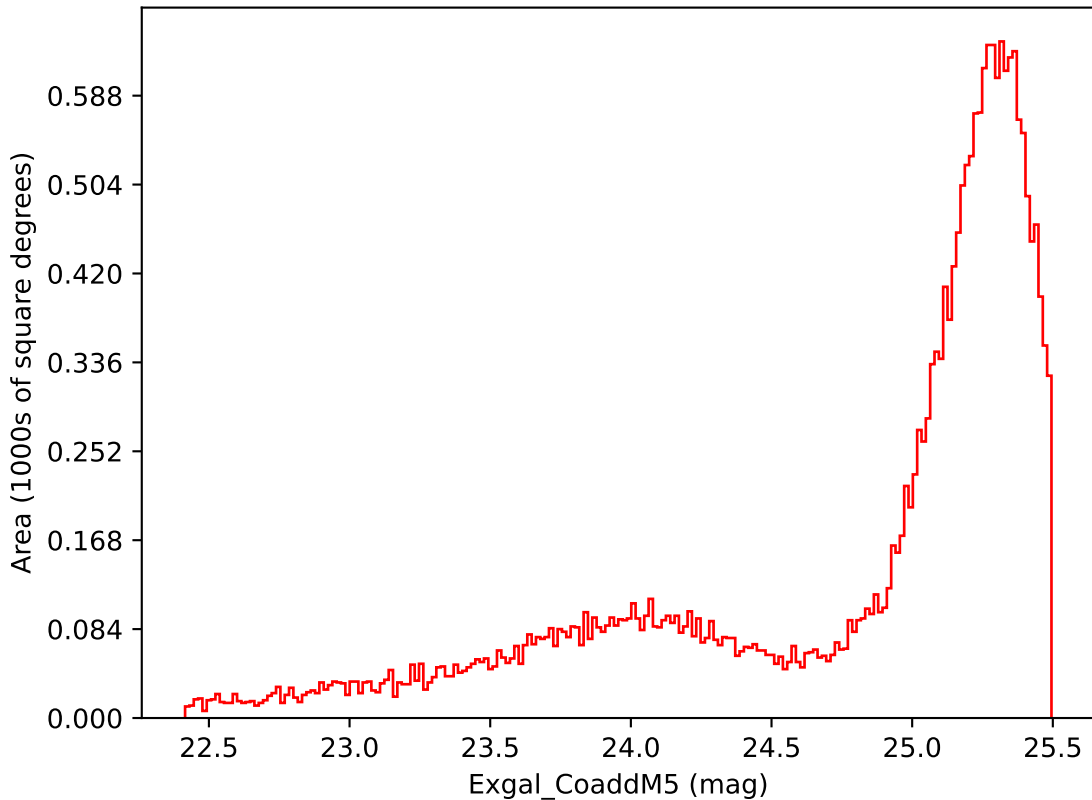
reweight_plane_v3.3_10yrs Yr 1 i band: Exgal_CoaddM5
