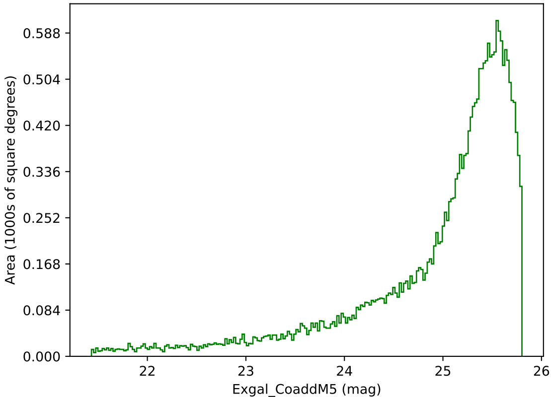
reweight_plane_v3.3_10yrs Yr 1 g band: Exgal_CoaddM5
