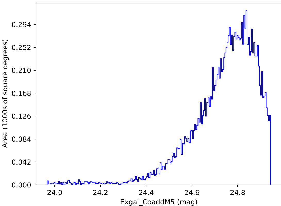
reweight_plane_v3.3_10yrs WFD y band: Exgal_CoaddM5
