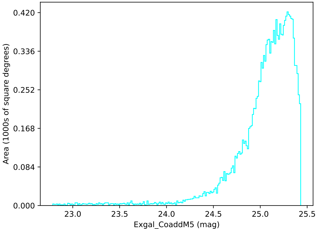
reweight_plane_v3.3_10yrs WFD u band: Exgal_CoaddM5
