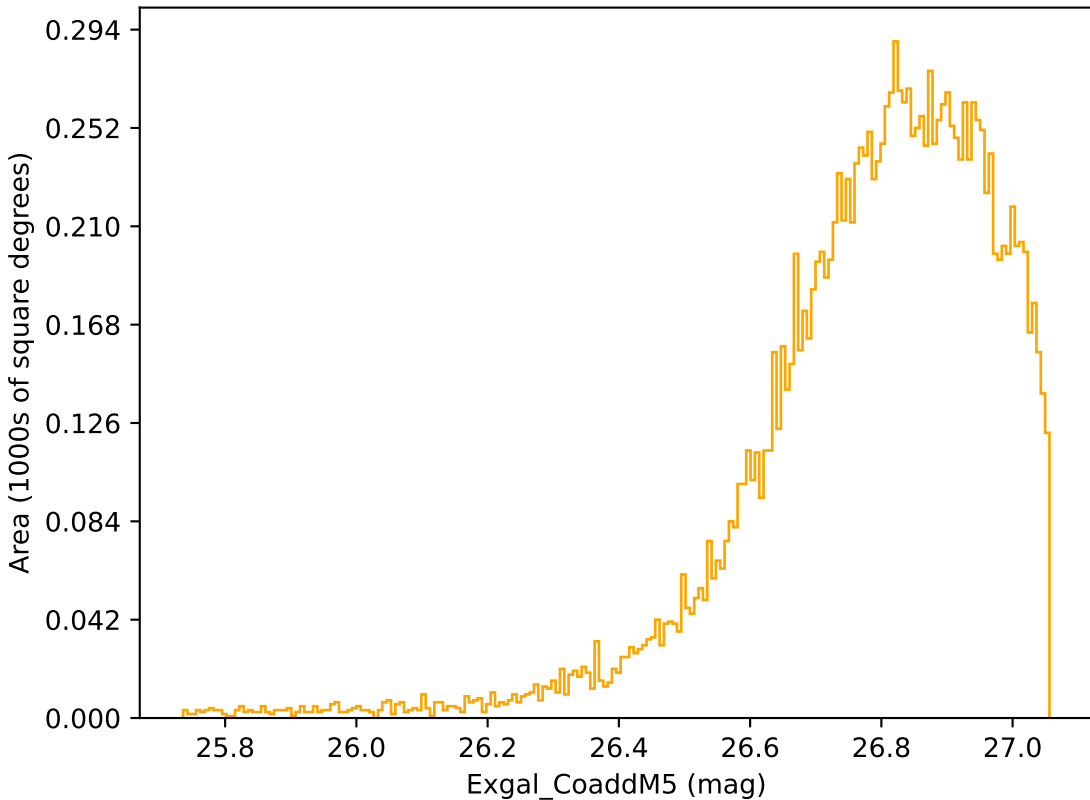
reweight_plane_v3.3_10yrs WFD r band: Exgal_CoaddM5
