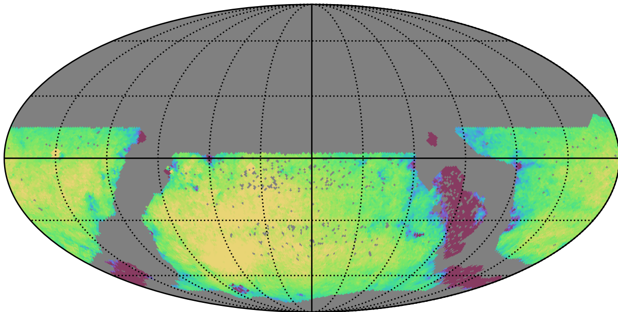
reweight_plane_v3.3_10yrs WFD g band: Exgal_CoaddM5
