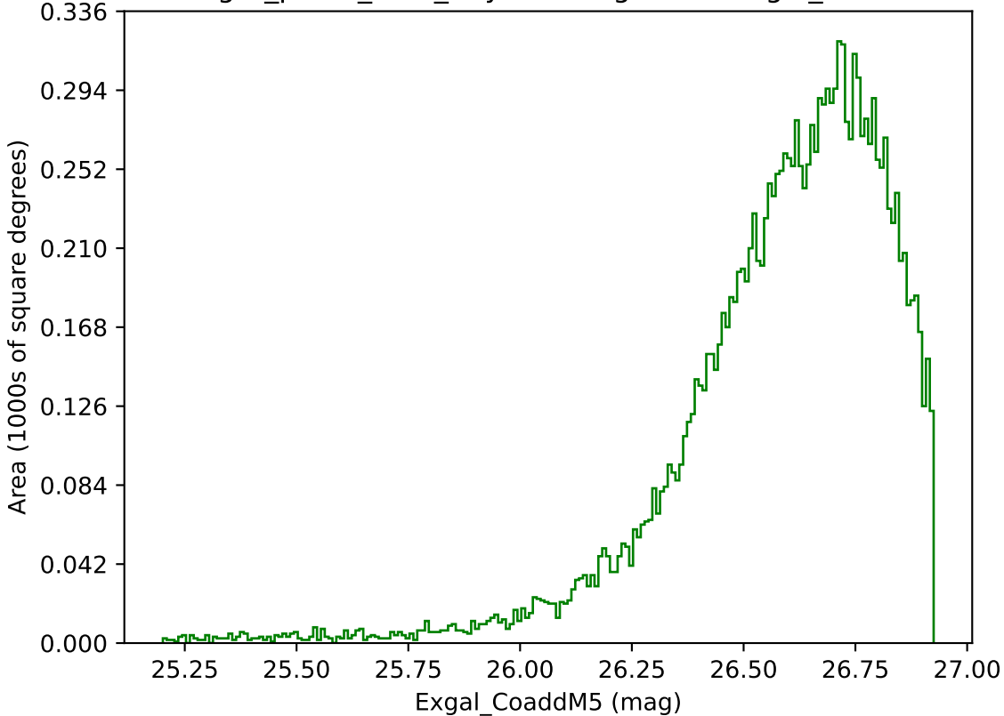
reweight_plane_v3.3_10yrs WFD g band: Exgal_CoaddM5
