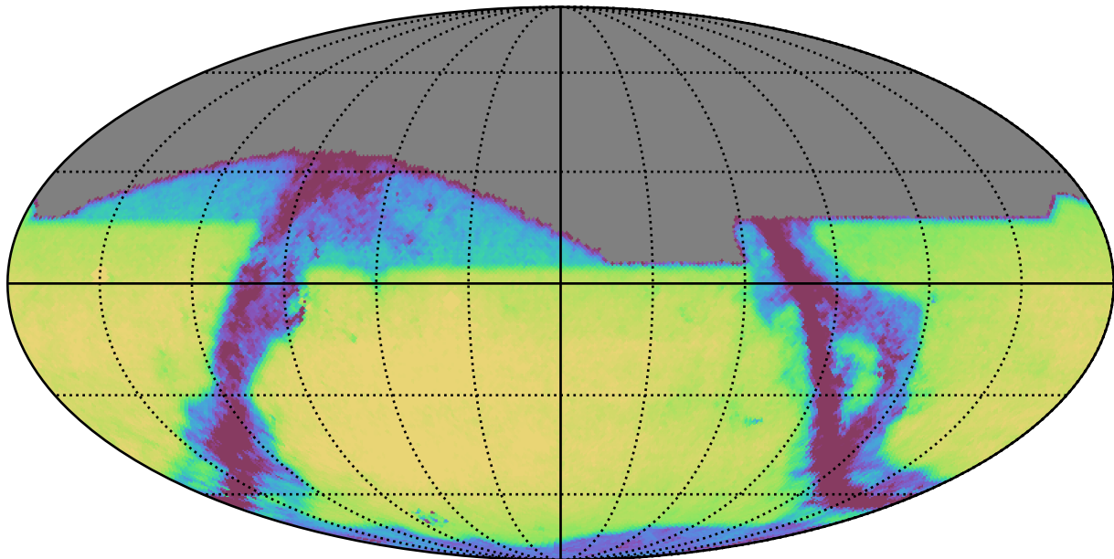
reweight_plane_v3.3_10yrs All sky z band: Exgal_CoaddM5
