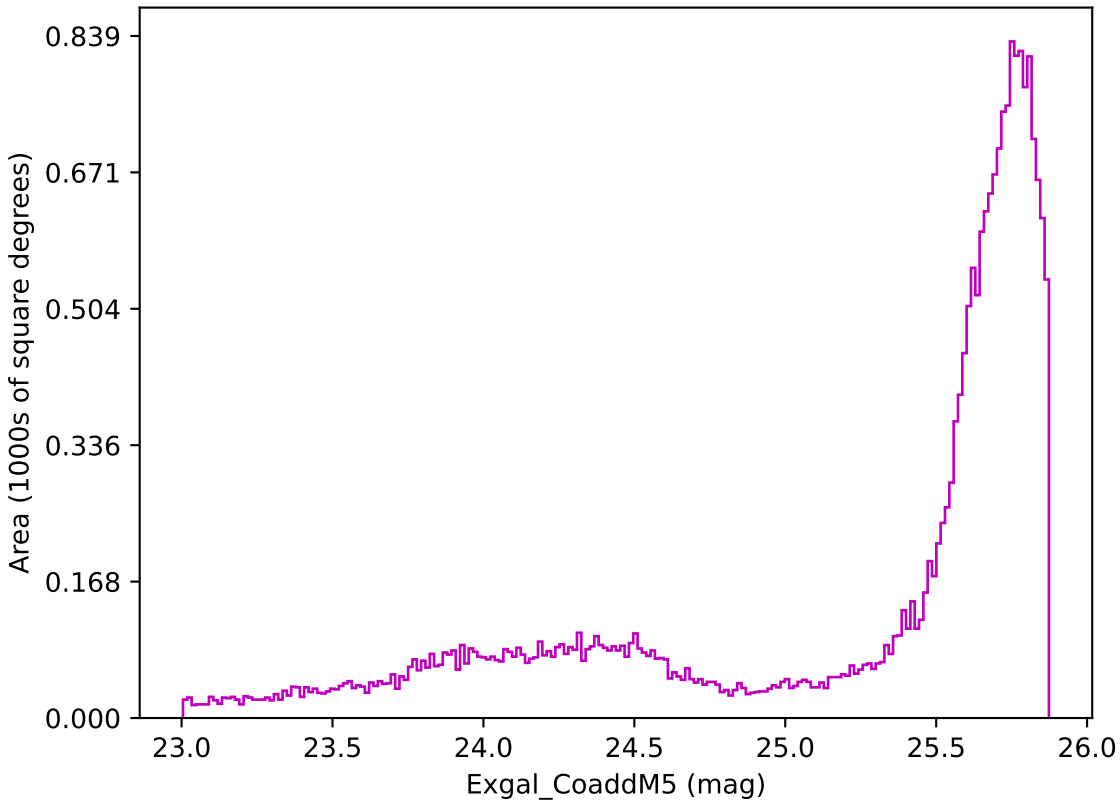
reweight_plane_v3.3_10yrs All sky z band: Exgal_CoaddM5
