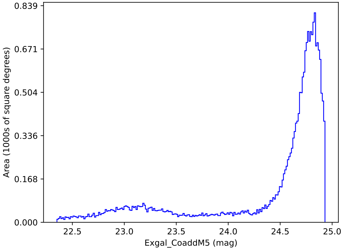
reweight_plane_v3.3_10yrs All sky y band: Exgal_CoaddM5
