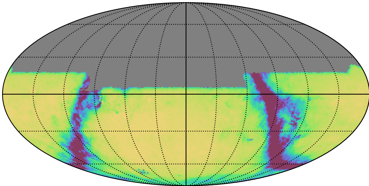
reweight_plane_v3.3_10yrs All sky u band: Exgal_CoaddM5
