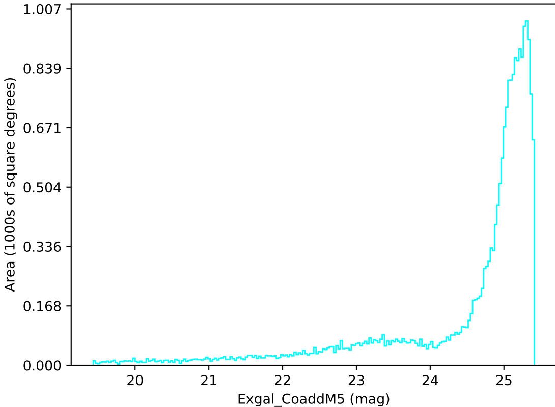
reweight_plane_v3.3_10yrs All sky u band: Exgal_CoaddM5
