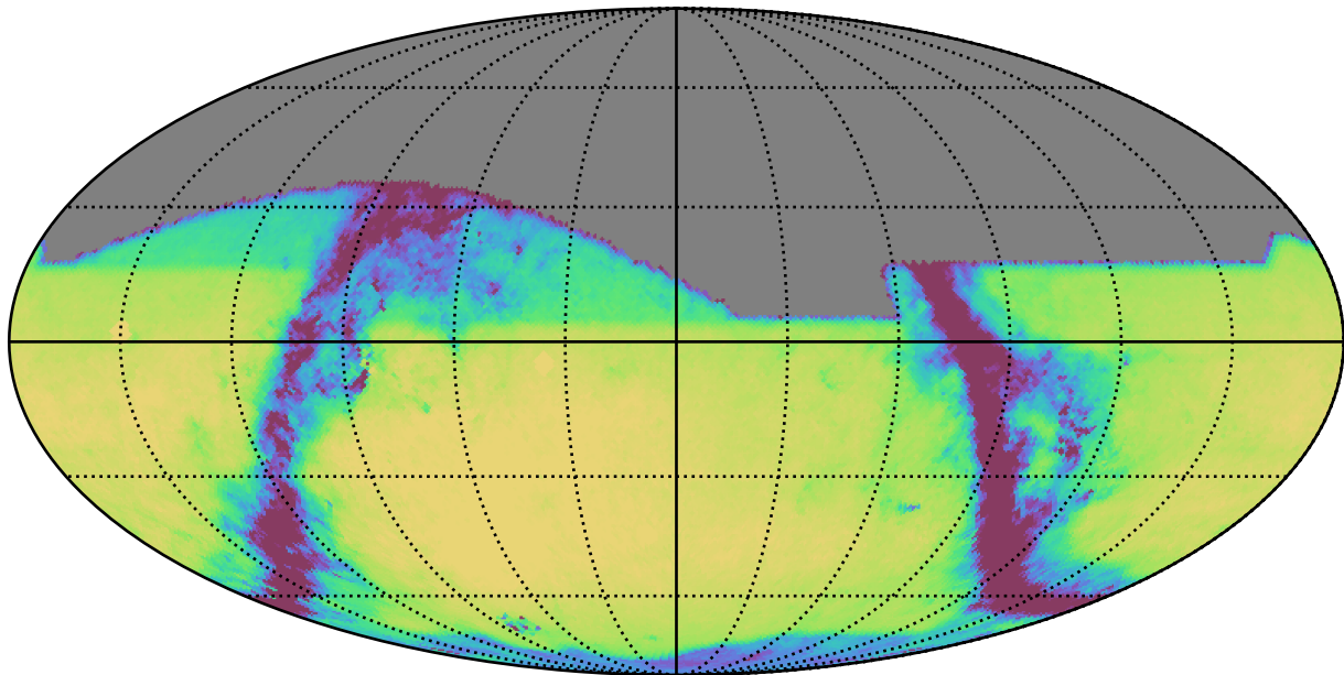
reweight_plane_v3.3_10yrs All sky r band: Exgal_CoaddM5
