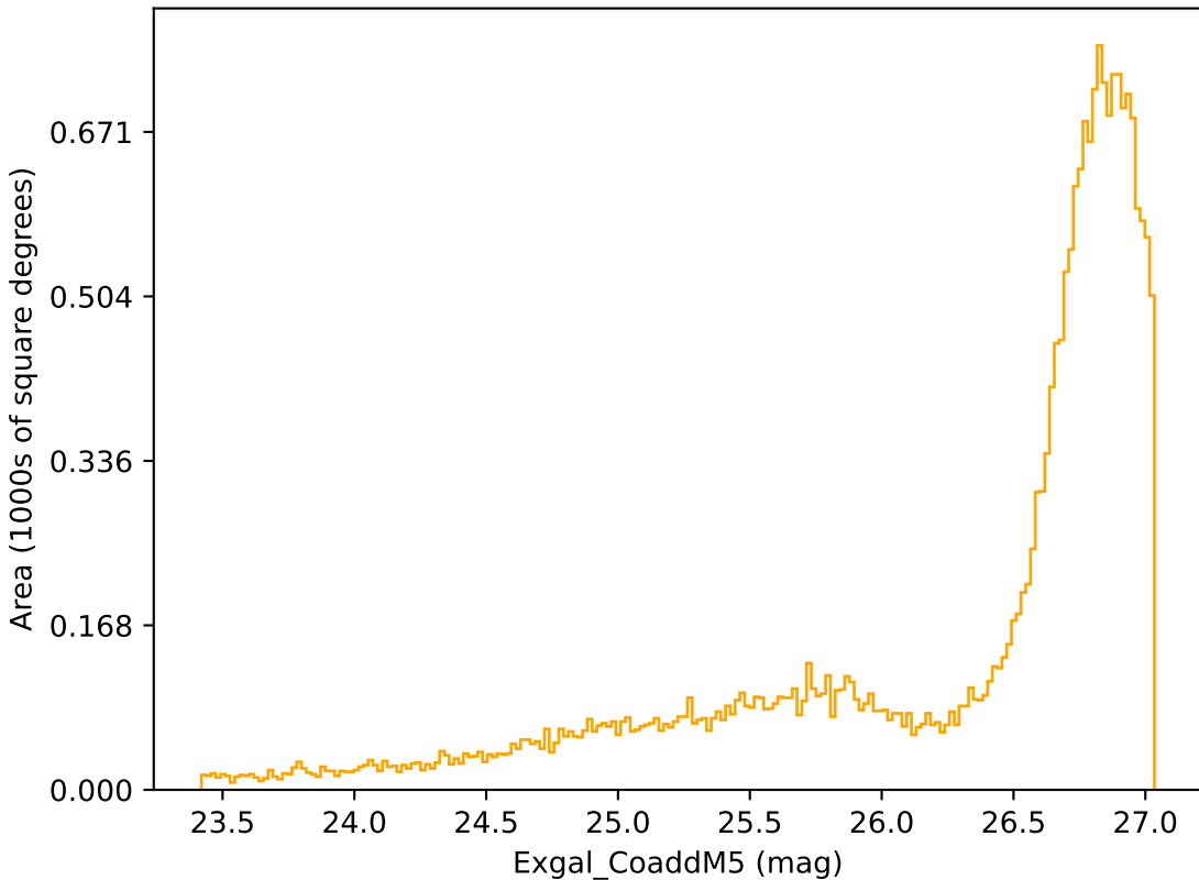
reweight_plane_v3.3_10yrs All sky r band: Exgal_CoaddM5
