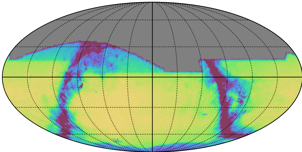
reweight_plane_v3.3_10yrs All sky i band: Exgal_CoaddM5
