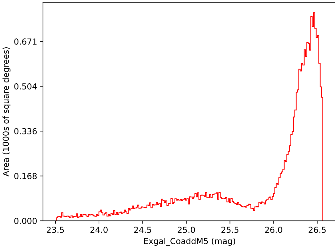
reweight_plane_v3.3_10yrs All sky i band: Exgal_CoaddM5
