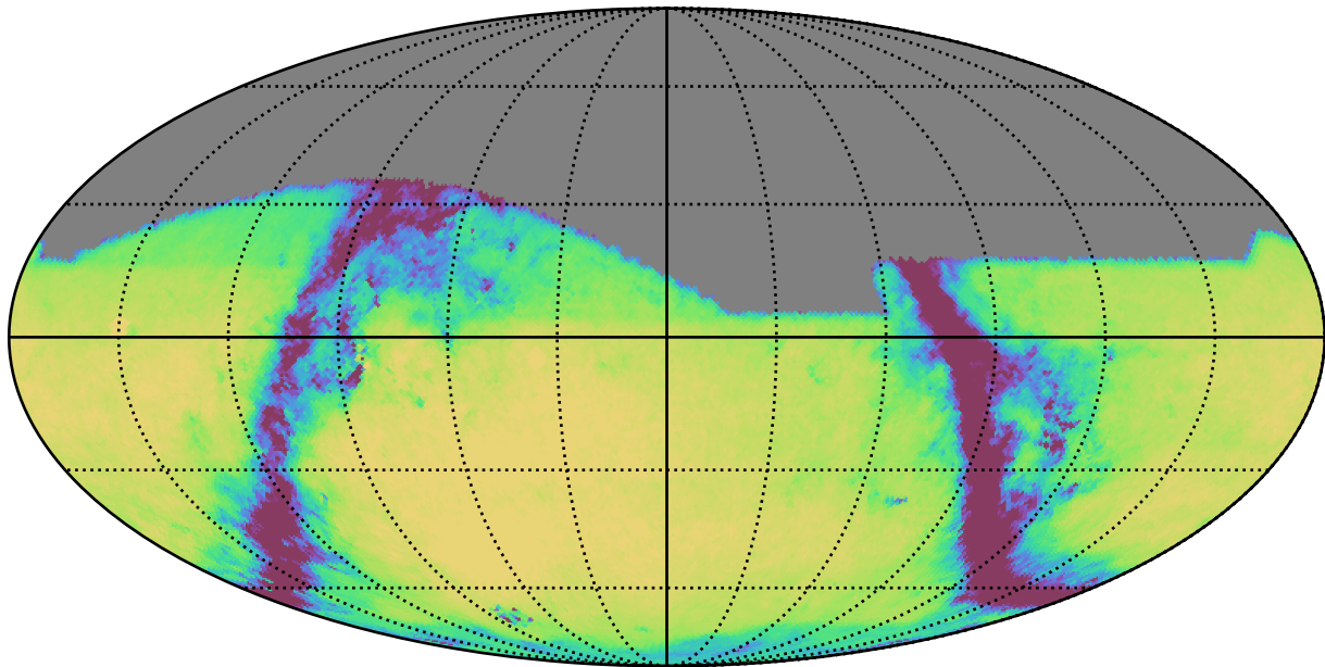
reweight_plane_v3.3_10yrs All sky g band: Exgal_CoaddM5
