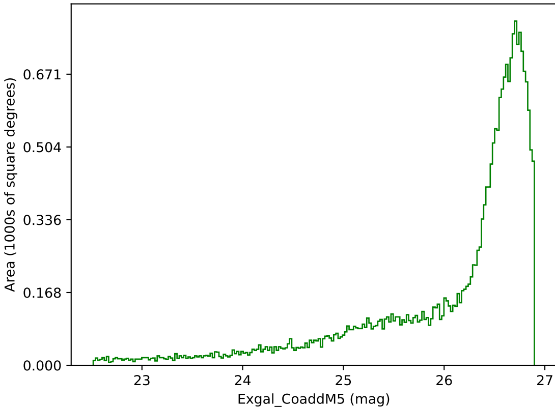
reweight_plane_v3.3_10yrs All sky g band: Exgal_CoaddM5
