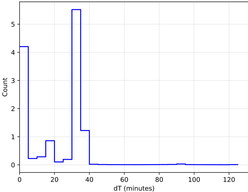
1e6reweight_plane_v3.3_10yrs All sky: DeltaT Histogram
